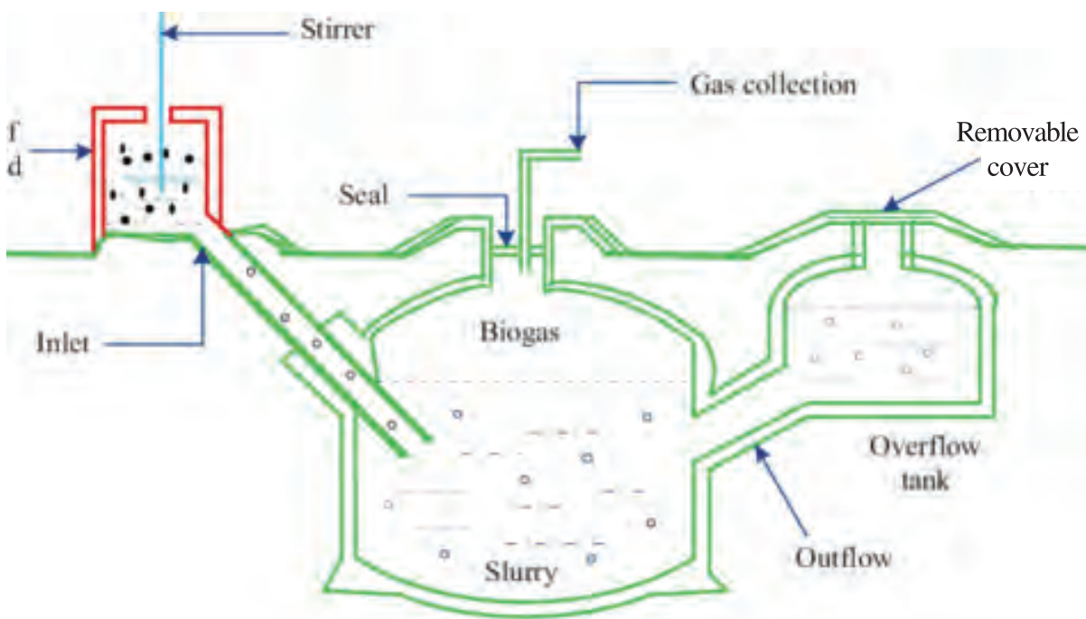
Fig 13.1 Biogas Plant
