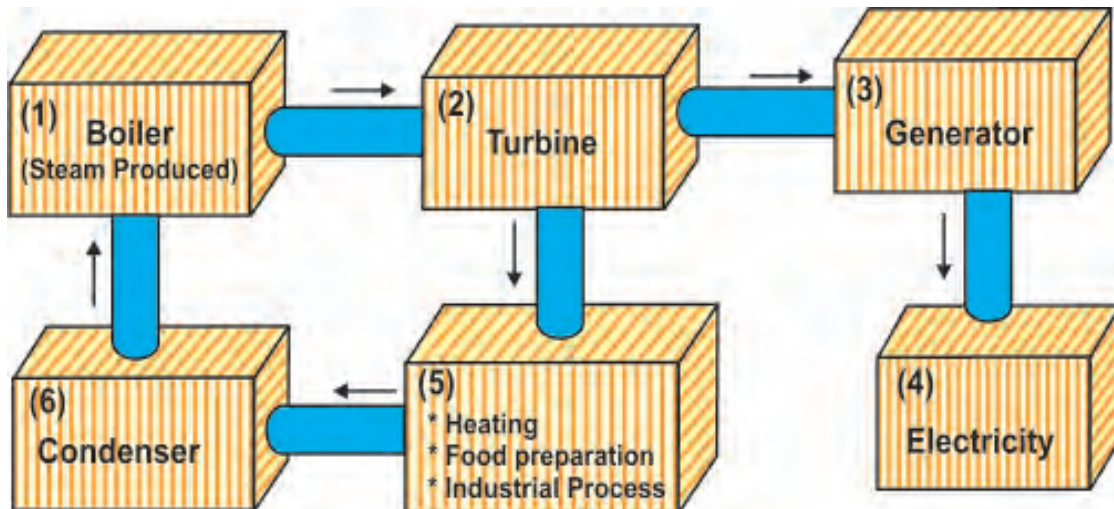
Fig 14.1 Cogeneration Unit
