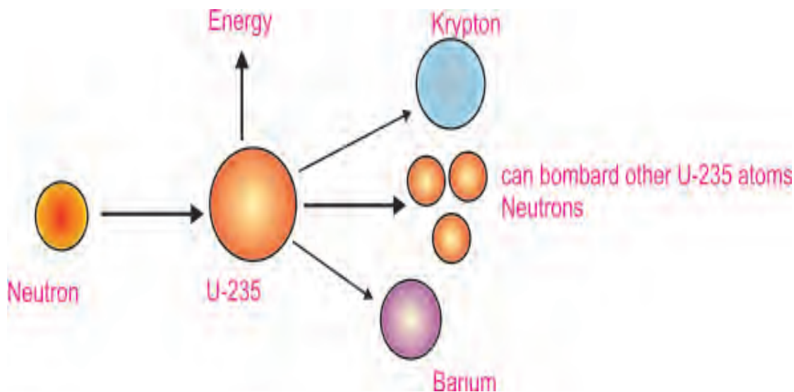
Fig 13.6 Nuclear Fission
